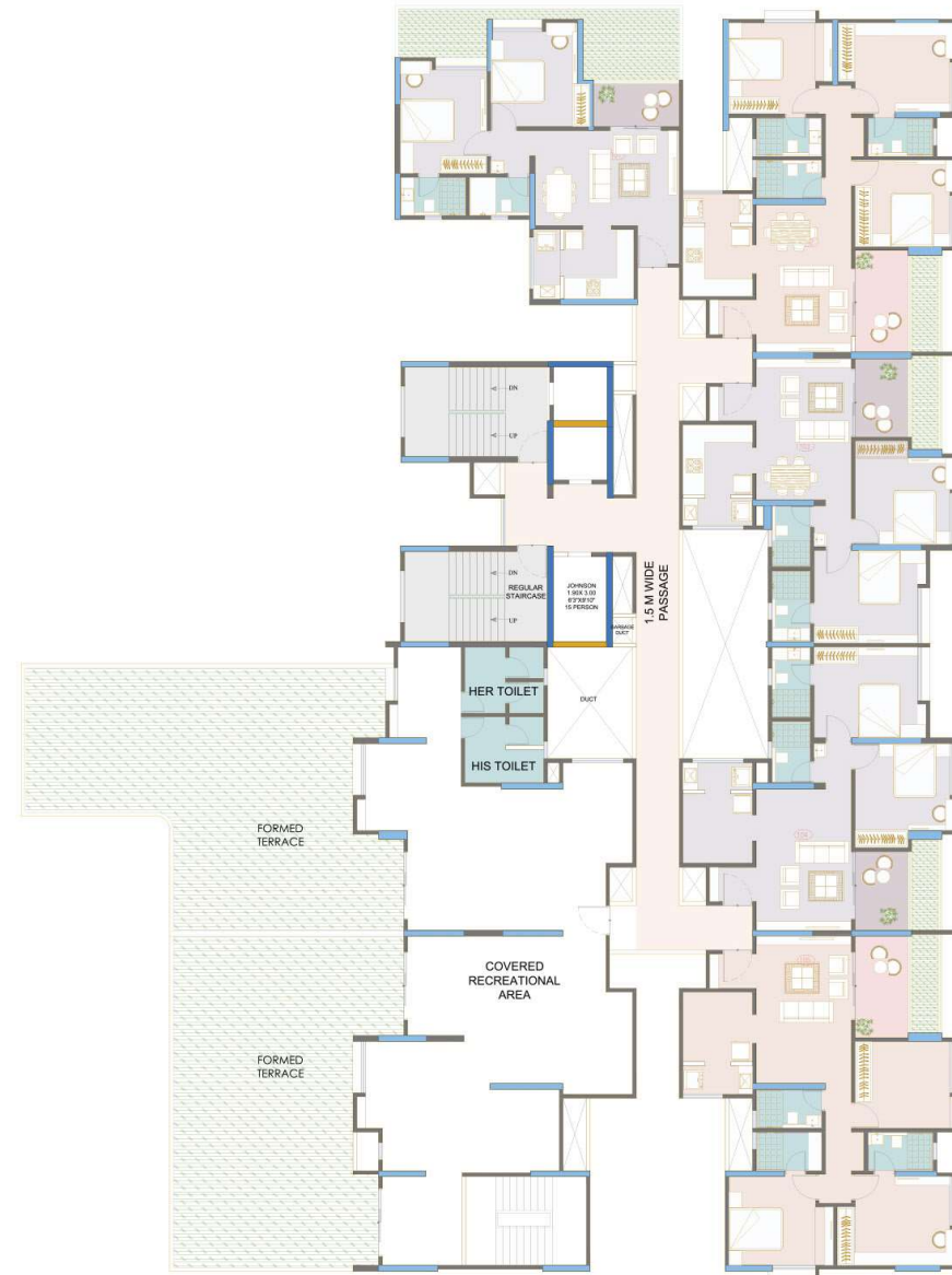
TYPICAL FLOOR PLAN FURNITURE LAYOUT
