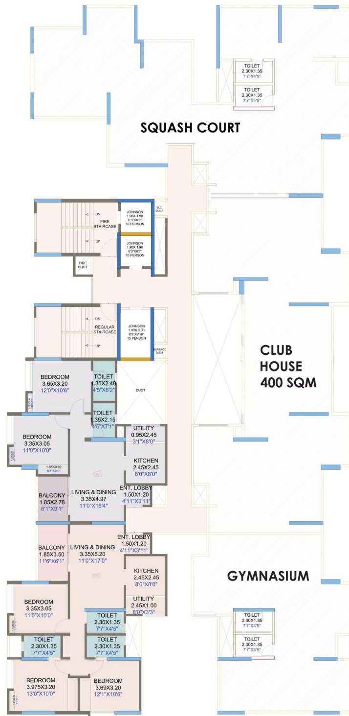
19TH FLOOR PLAN
